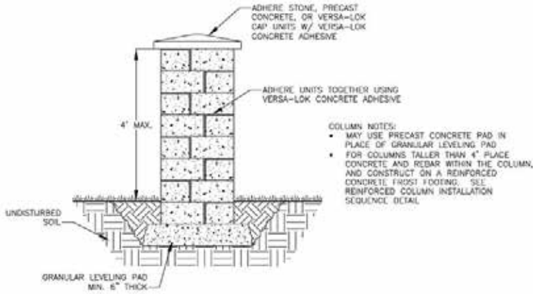
20" STANDARD COLUMN SECTION STANDARD-UNREINFORCED COLUMN (4' TALL MAX.) SCALE: NONE
